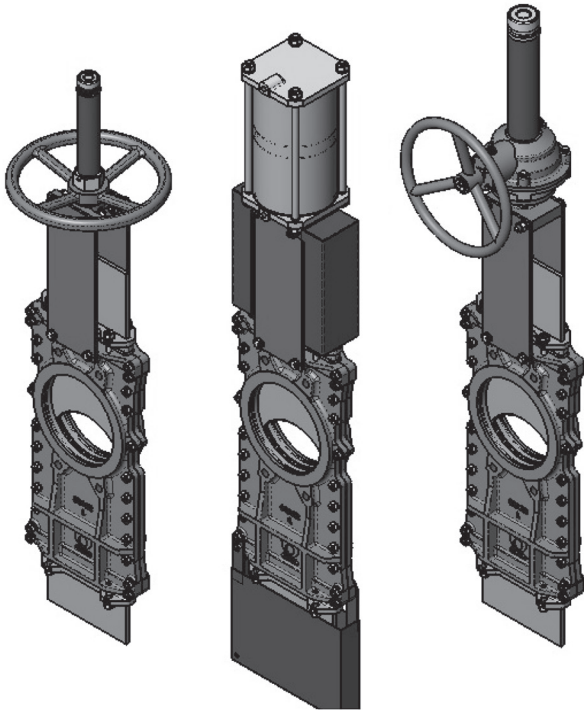
Handwheel actuator
