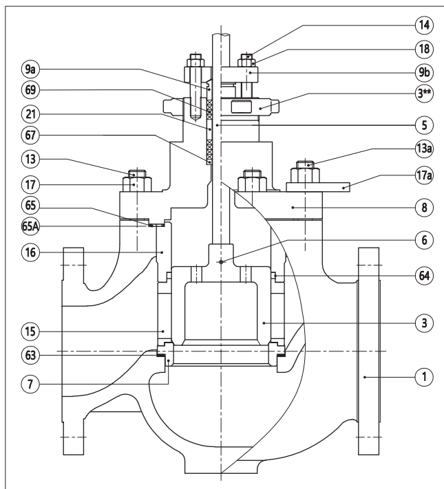
Fig. 8 Conventional Cage-Balance Trim
