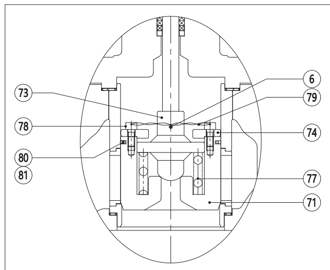
Fig. 9 Pilot balance trim
